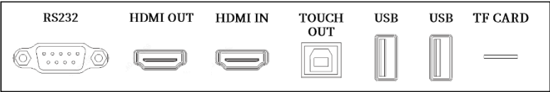
Front Interfaces
